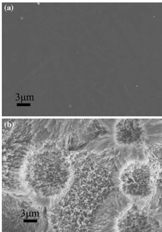
Fig. 10 Surface structures of PHB on SEM. (a) Without cell inoculation (b) With cell inoculation HS 45-1
