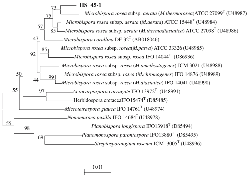
Fig. 3 The phylogenetic tree based on the 16S rRNA gene sequences of the isolate HS 45-1
