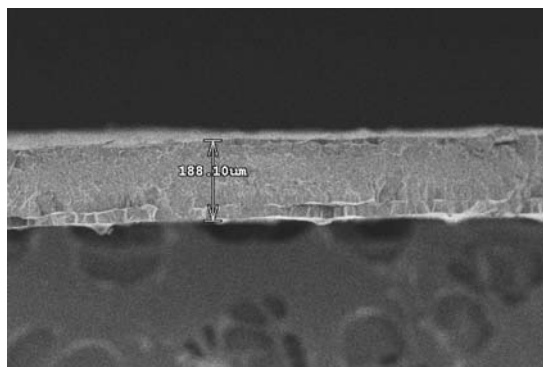
Fig. 2 Scanning electron micrographs of PES film thickness
